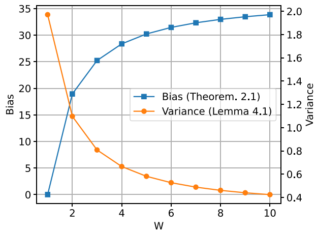
Fig. 1 Trend of the bias (Theorem 2.1) and variance (Lemma 4.1) bounds for different values of W \in \{1, 2, \dots, 10\} . Exemplification with \gamma = 0.9 , H = 10 , N = 100 and a stochasticity index D(P) = 0.1
