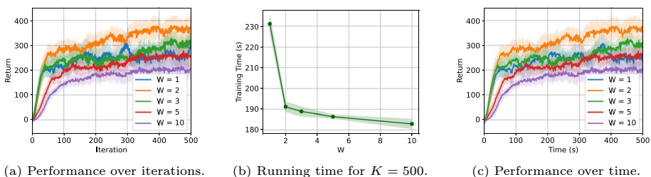
Fig. 4 Learning curves and training time for Half-Cheetah (10 runs, mean \pm 95% C.I.)
