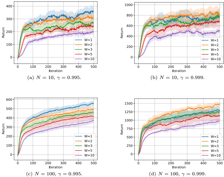
Fig. 12 Learning curves for Half-Cheetah with H = 700 (10 runs, mean \pm 95% C.I.)
