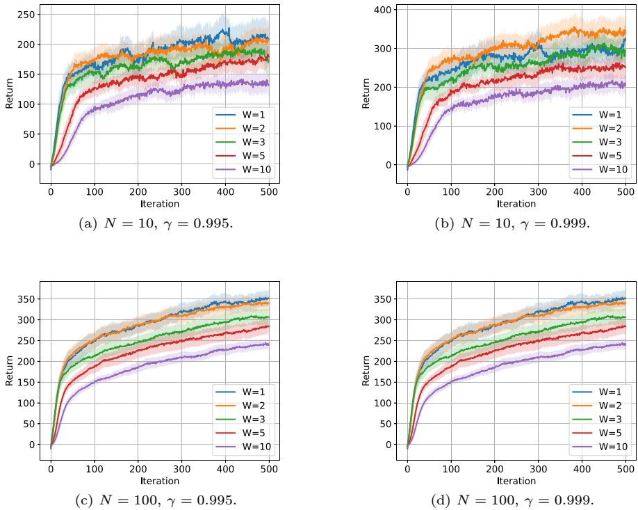
Fig. 10 Learning curves for Half-Cheetah with H = 200 (10 runs, mean \pm 95% C.I.)
