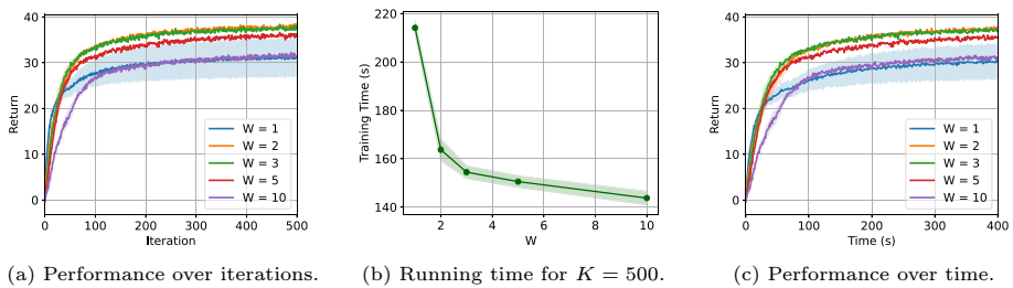
Fig. 3 Learning curves and training time for Swimmer (10 runs, mean \pm 95% C.I.)
