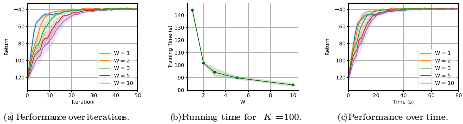
Fig. 2 Learning curves and training time for the dam control task (10 runs, mean \pm 95% C.I.)
