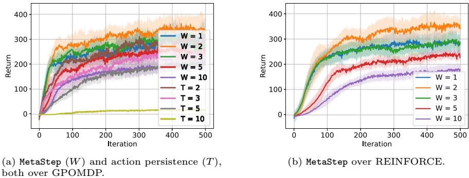
Fig. 13 Learning curves for Half-Cheetah with H = 200 , \gamma = 0.999 and N = 10 (10 runs, mean \pm 95% C.I.)
