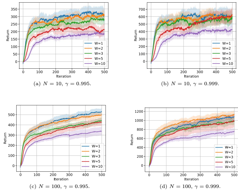
Fig. 11 Learning curves for Half-Cheetah with H = 500 (10 runs, mean \pm 95% C.I.)
